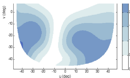
Hybrid Digital Free Form Sun with Frame wrap of 0°
